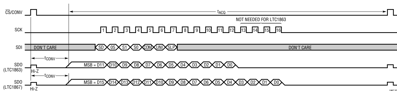
Figure 7. Example 2, \overline{\text{CS}}/\text{CONV} Starts a Conversion with Short Active HIGH Pulse. With \overline{\text{CS}}/\text{CONV} Returning LOW Before the Conversion, the ADC Remains Powered Up.
